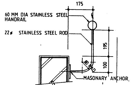
DETAIL OF SAFETY RAIL ADJACENT TO LOT 762
