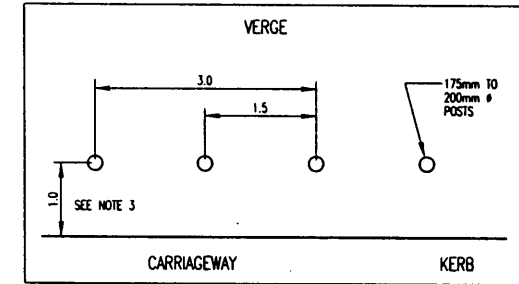
BOLLARD DETAIL NOT TO SCALE
