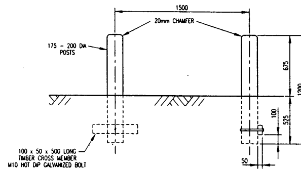
TIMBER STRUT NOT TO SCALE
