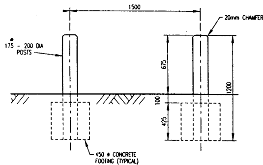
CONCRETE FOOTING NOT TO SCALE
