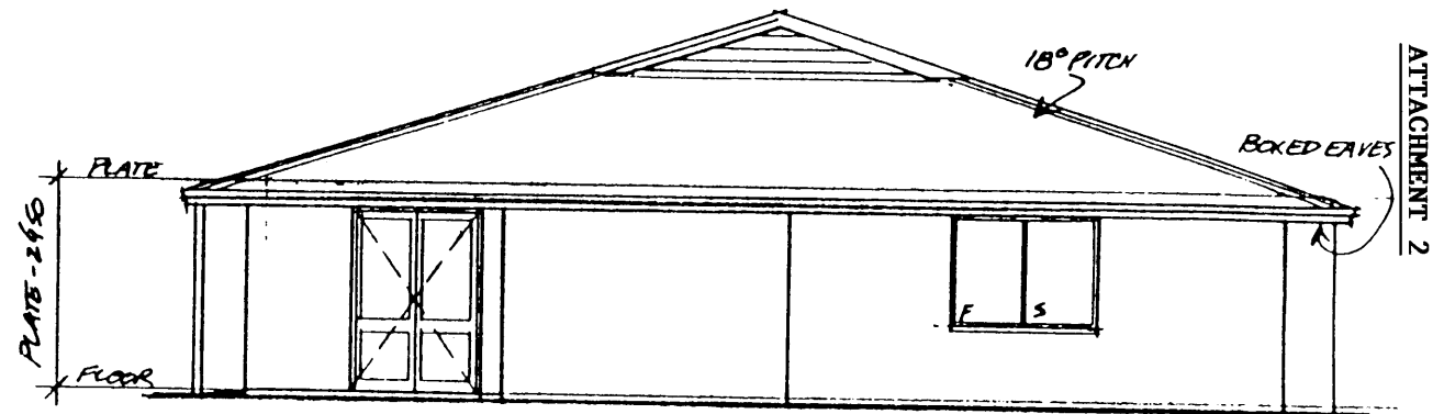
FRONT ELEVATION 1:100
