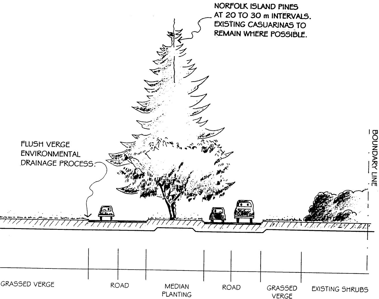
MARMION AVENUE CROSS SECTION AT SORRENTO DUNCRAIG RECREATION CENTRE
