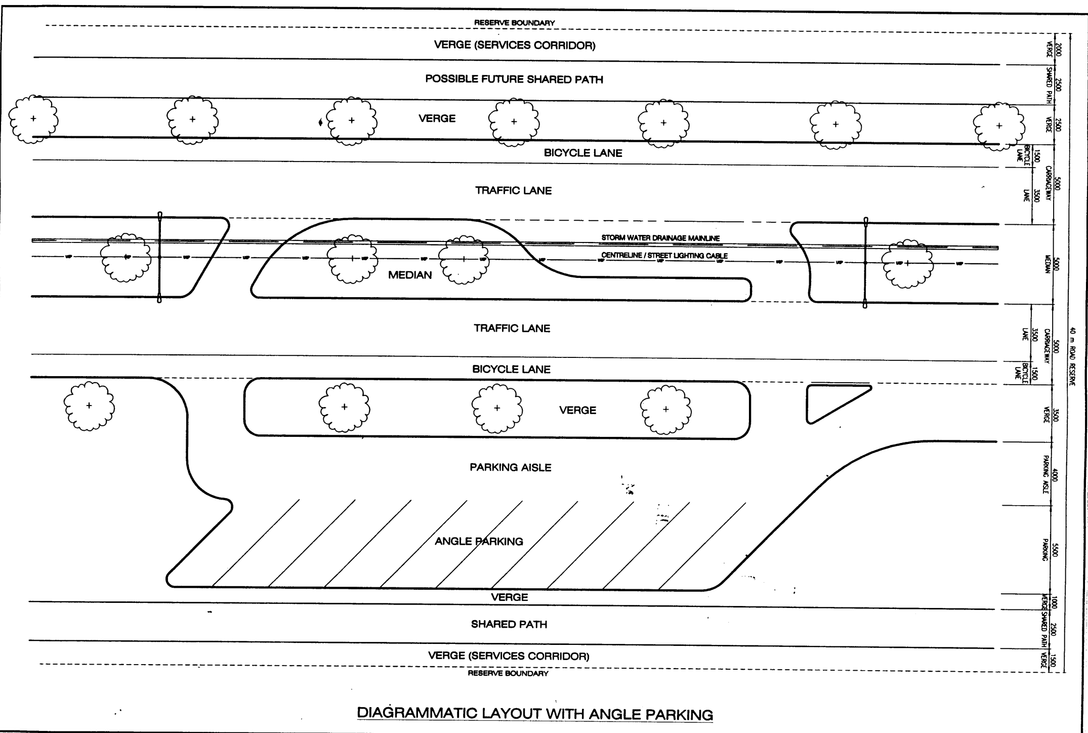
OCEAN REEF ROAD SINGLE LANE BOULEVARD
