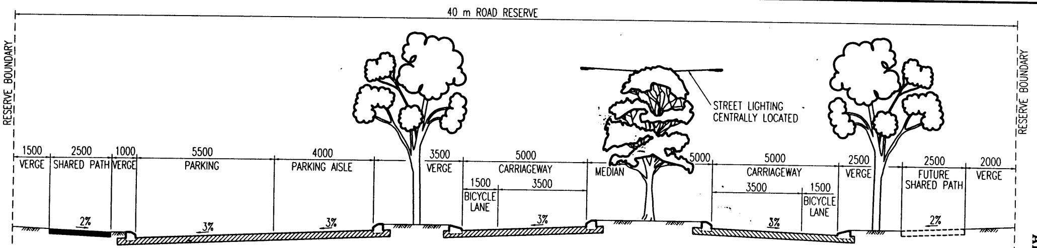
FIRST STAGE CROSS SECTION
