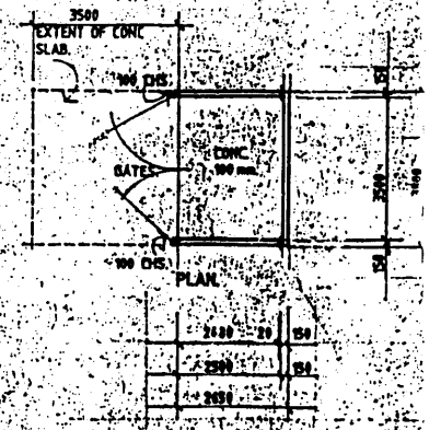
1:100, BIN ENCLOSURE, DL
