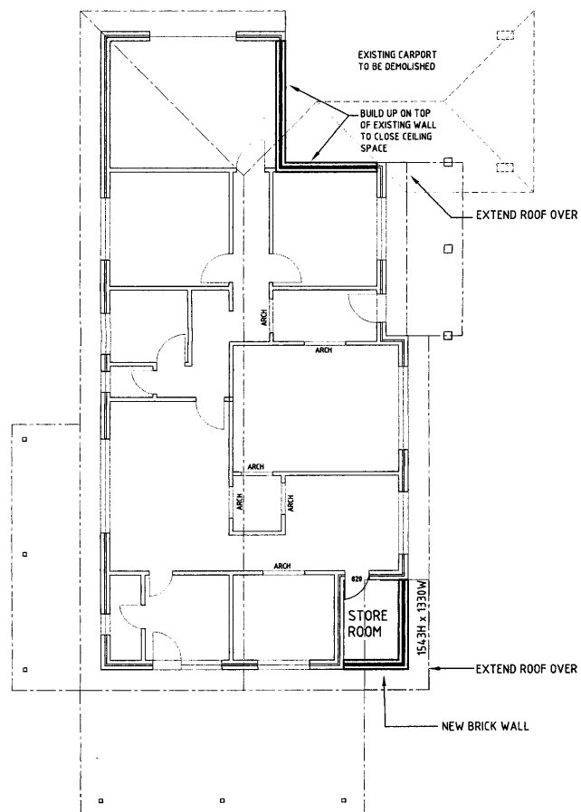
FLOOR PLAN 1:100
