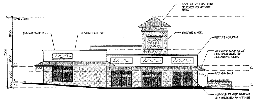
EAST ELEVATION (CARPARK)
