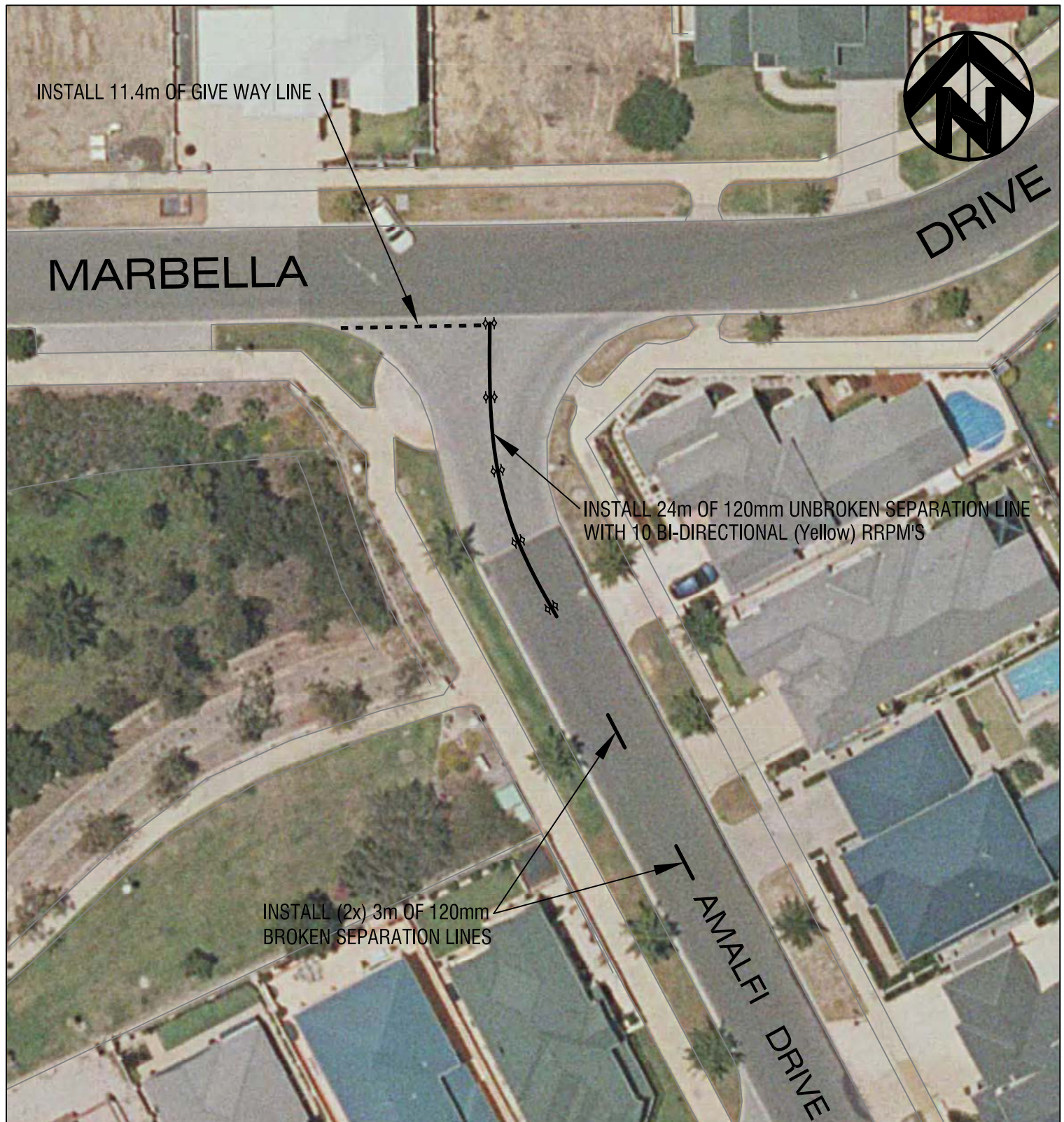
MARBELLA DRIVE / AMALFI DRIVE - PROPOSED LINE MARKING PLAN
