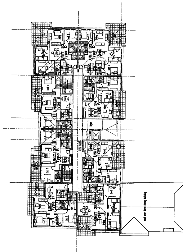
THIRD FLOOR PLAN 1:200
