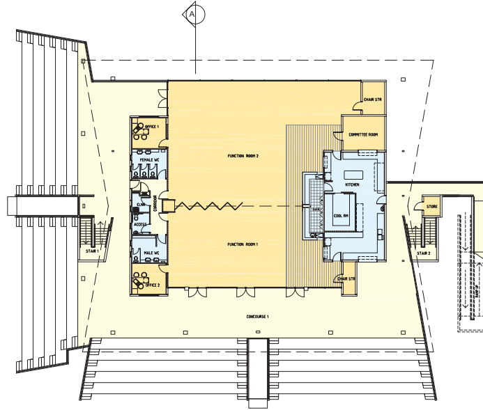
FIRST FLOOR PLAN 1:200 @ A1
