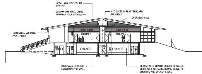
SECTION A 1:200 @ A1
