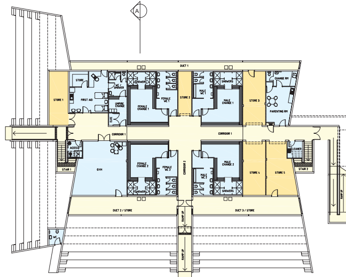
GROUND FLOOR PLAN 1:200 @ A1
