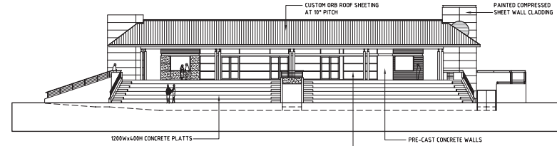
SOUTH ELEVATION 1:200 @ A1
