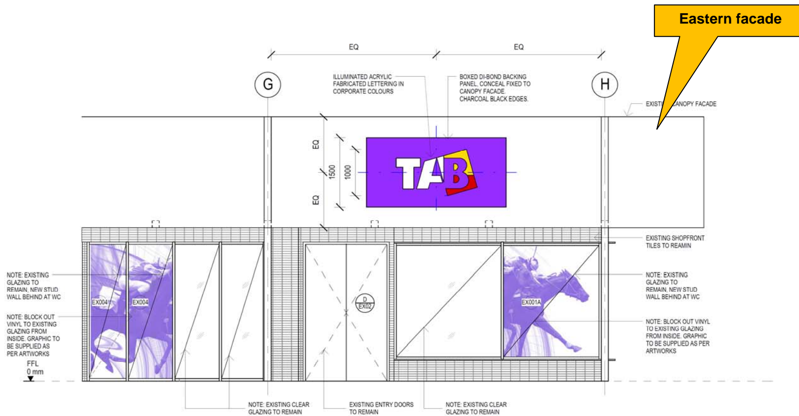
1 SHOPFRONT ELEVATION 3 - FROM ROAD A721 1:50
