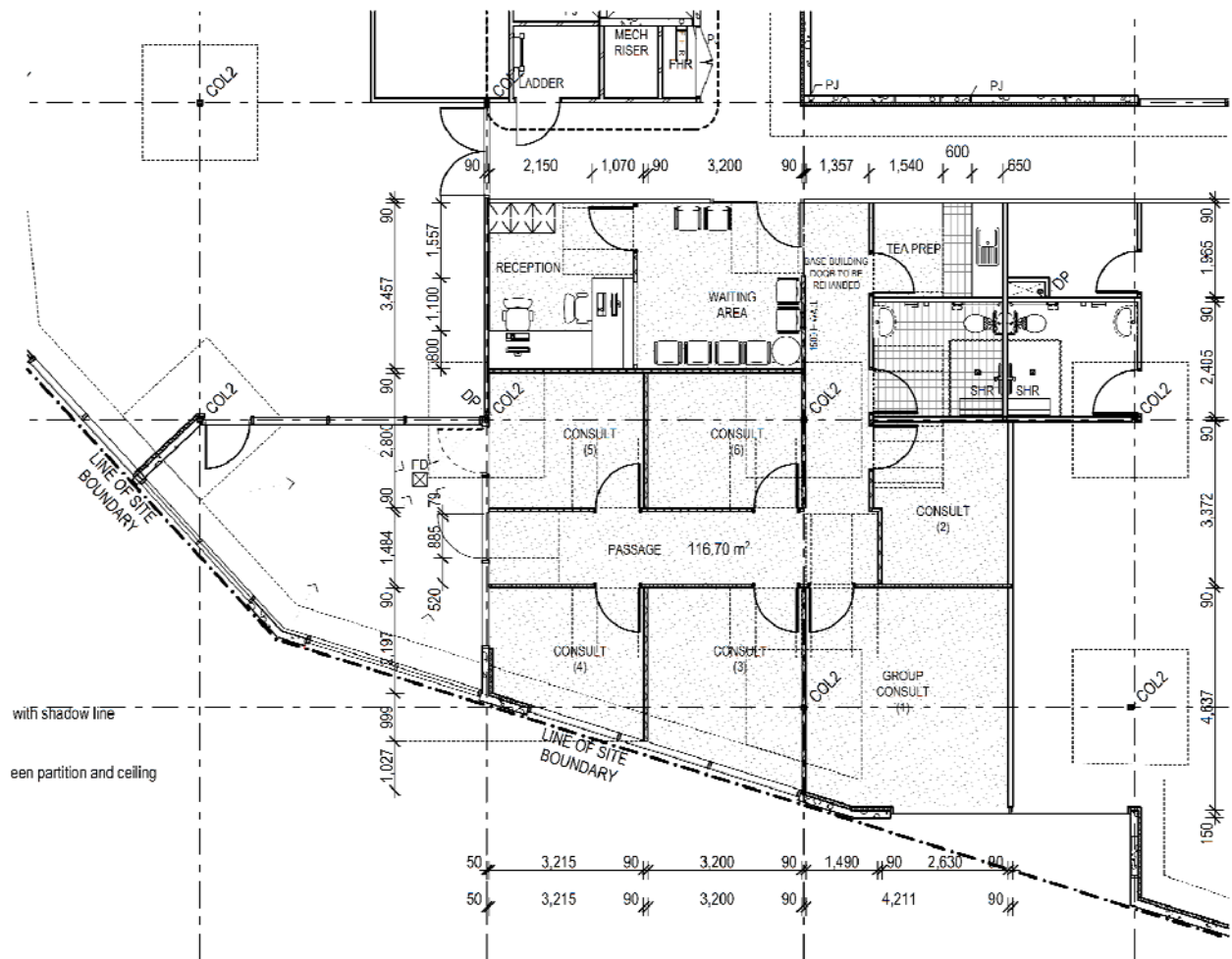
1 SUITE 12 SKETCH PLAN Scale 1:100
