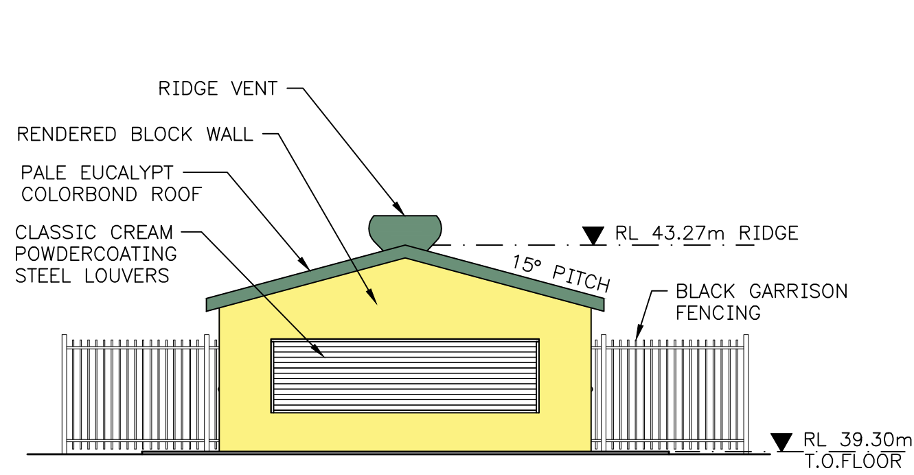
VIEW A 003
