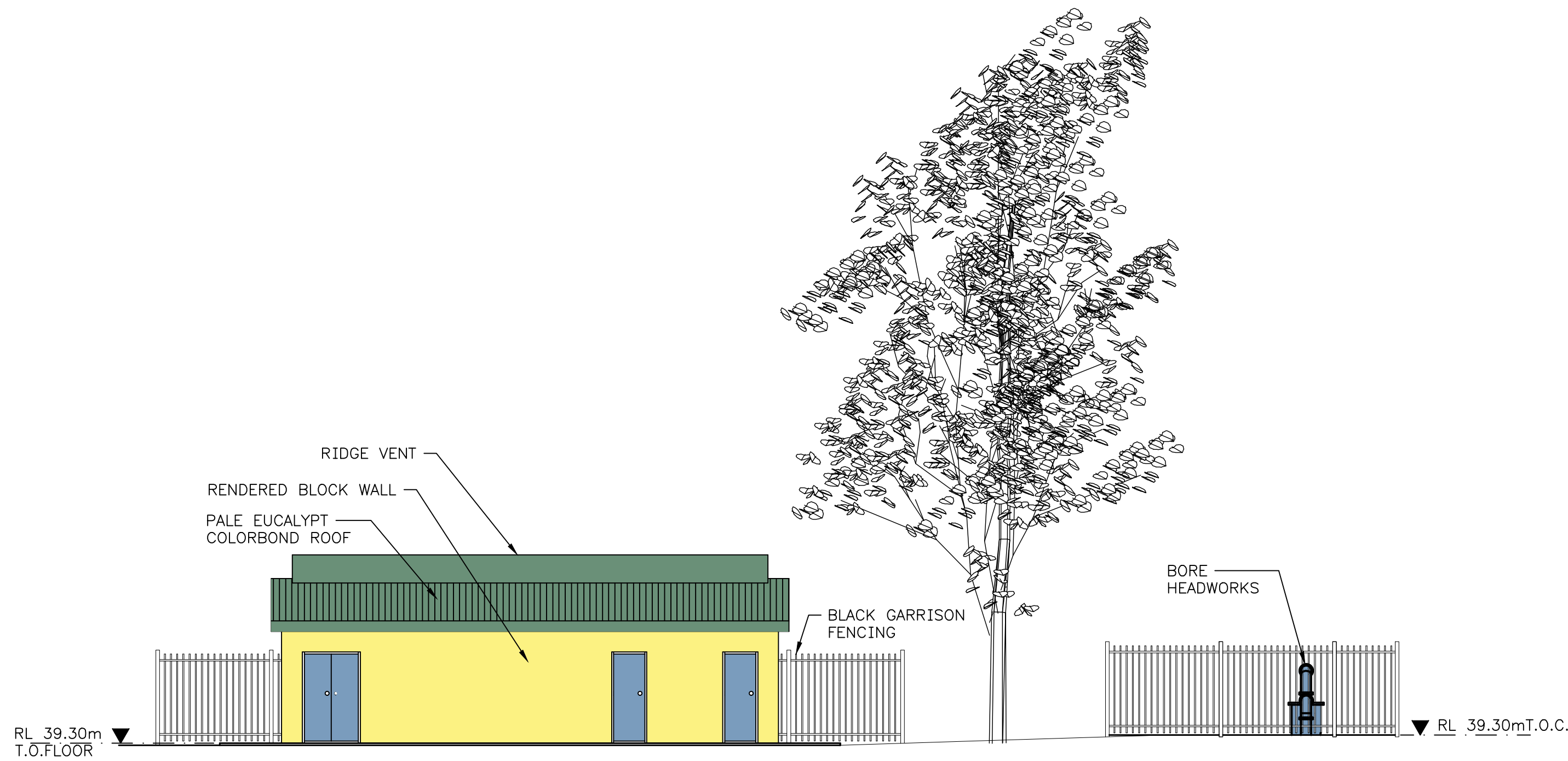
VIEW B 003
