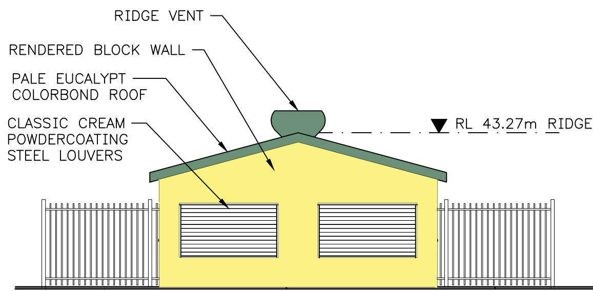
VIEW C 003
